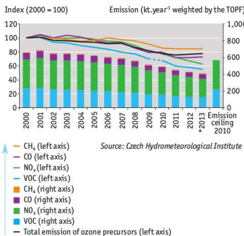
Chart 1 → Total emissions of ozone precursors in the Czech Republic and the levels of the national emission ceilings (for VOC and NO x ) for 2010 [index, 2000 = 100]; [kt. year -1 weighted by the TOPF], 2000–2013
